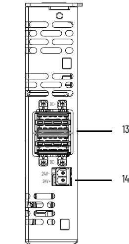
ArmorKinetix PIM, Top View
