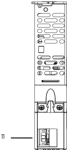
ArmorKinetix PIM, Bottom View
