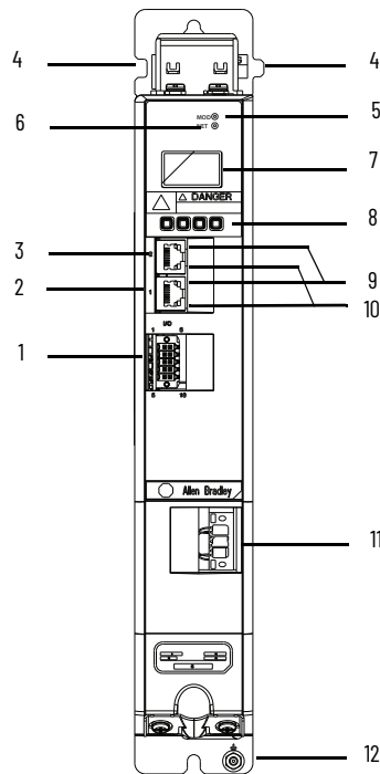
ArmorKinetix PIM, Front View
