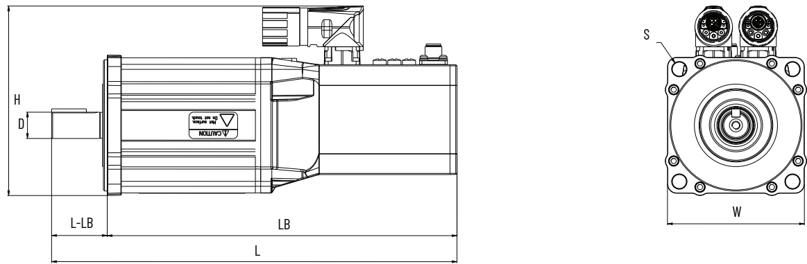
DSM Module Dimensions Table, 115 mm Frame Size
